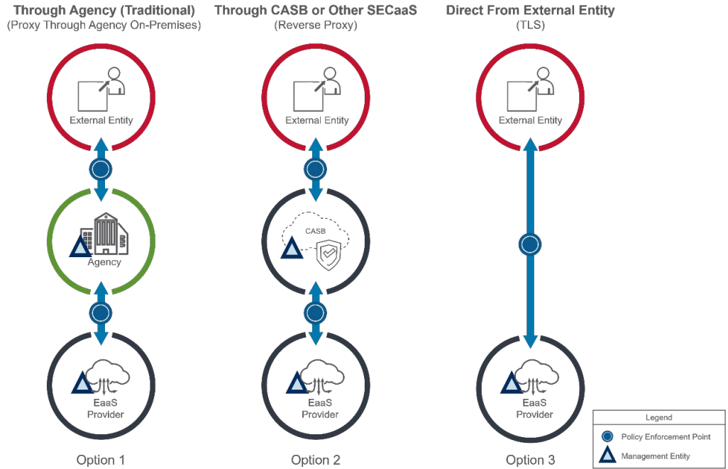
Figure 14: Security Pattern 3 - External Entity to Agency Email Service
